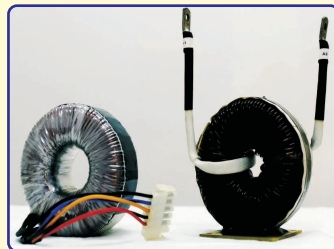
High Power Toroidal Transformer, Inductor
