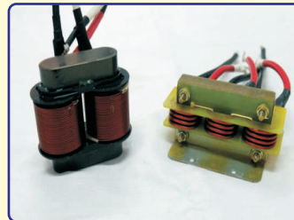
Complex Edge winding choke
