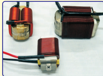
Edge Winding Amorphous Chokes
