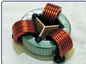
Complex Edge Winding Chokes
